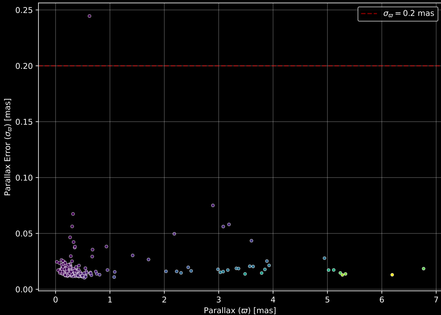
APOGEE DR17 Field: [240+04] Parallax Quality (n= 315)
