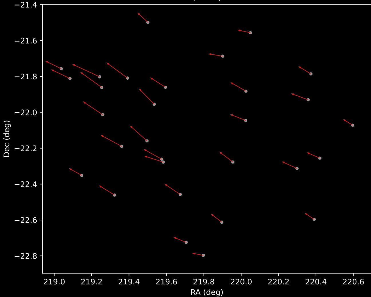
APOGEE DR17 Cluster 6 Proper Motion Vectors (n=30)
